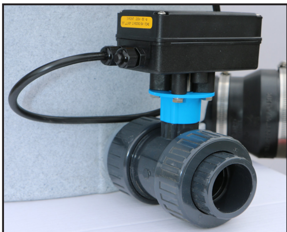
1 1/2" AUTOMATED WASTE VALVE (Factory fitted to EazyPod)
